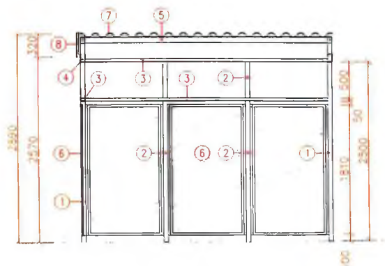
REZ A 1:50
